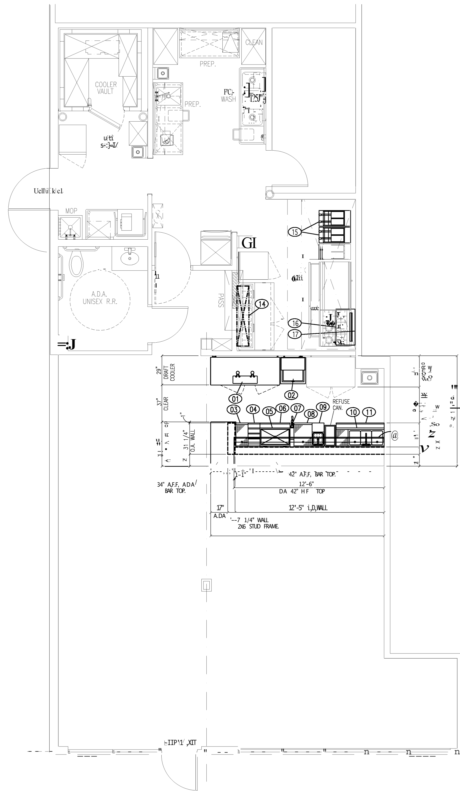
PROPOSED BAR AREA RENOVATION LAYOUT SCALE: 1/4" = 1'-0"
