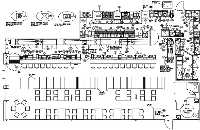
1 FOOD & BAR FACILITIES ARRANGEMENT PLAN K1 SCALE: 1/4" = 1'-0" SCALE: 1/4" = 1'-0"
