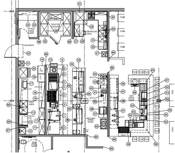
01 floor plan 1/8" = 1'-0"
