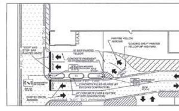
ENLARGED CUSTOMER LOADING CANOPY SCALE - 1'-3"0"
