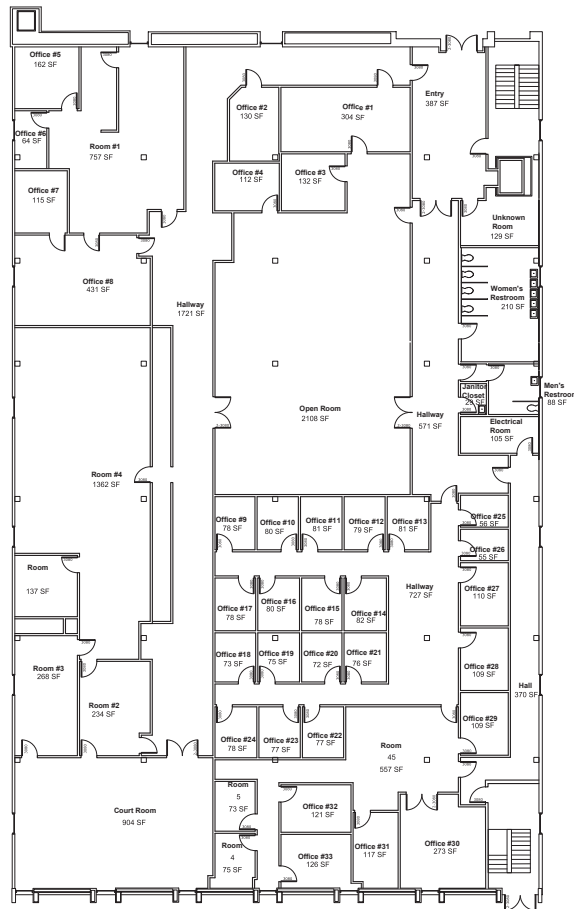
1st FLOOR: SCALE: 3/32" = 1'-0"
