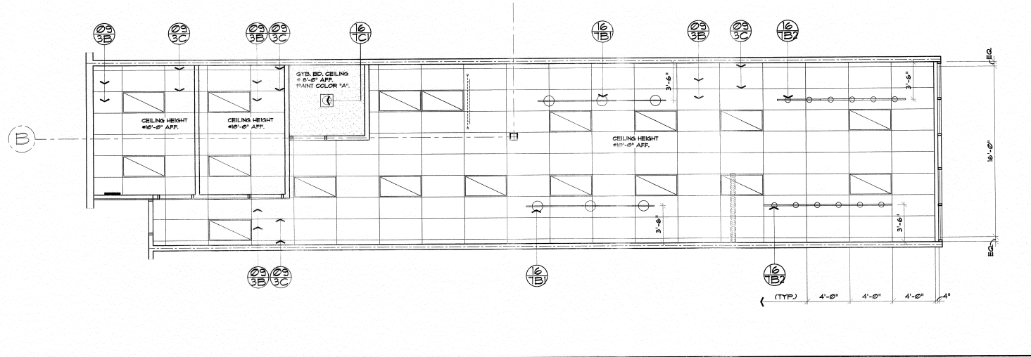
2 REFLECTED CEILING PLAN 1/4" = 1'-0"
