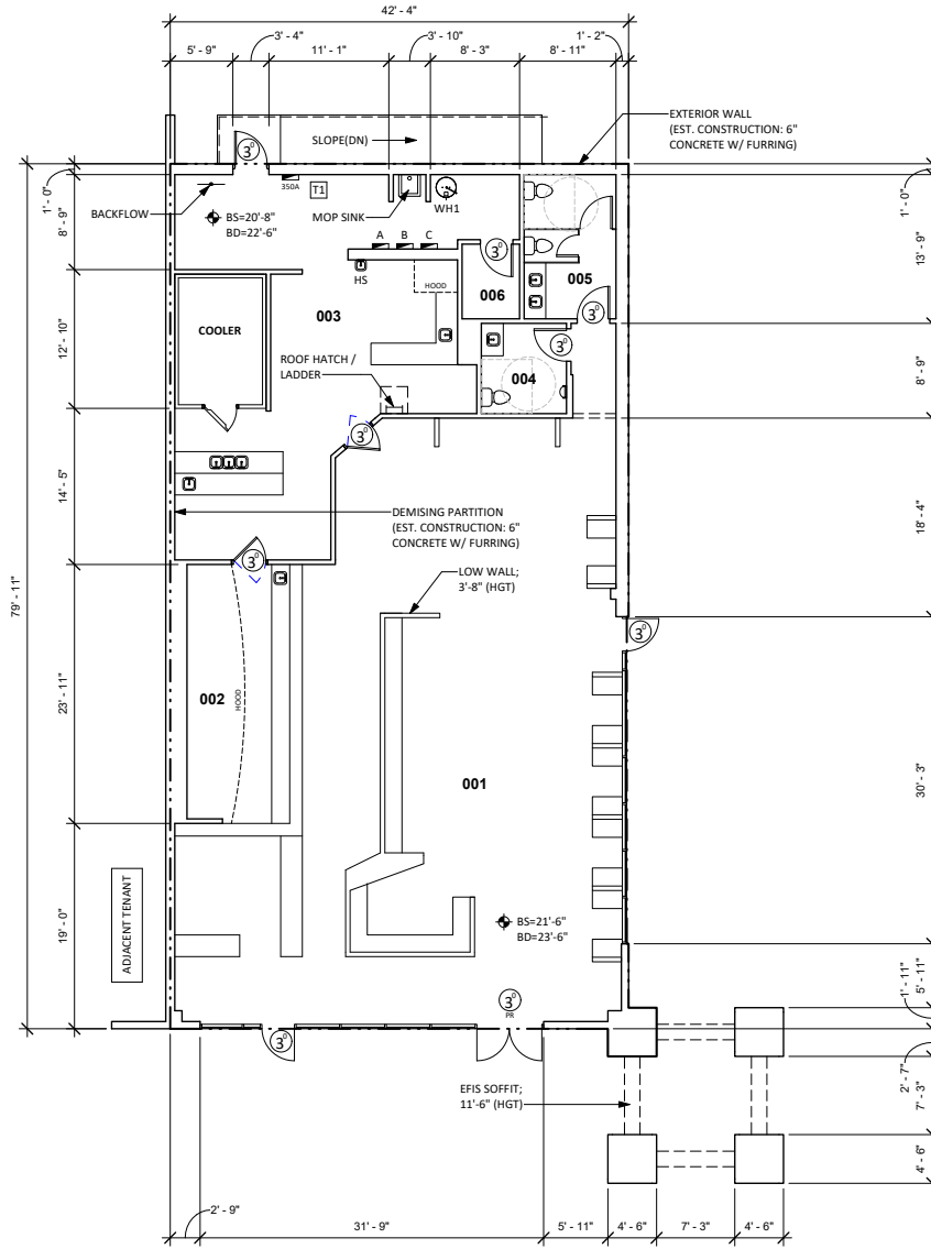
④ EXISTING FLOOR PLAN 1/8" = 1'-0"
