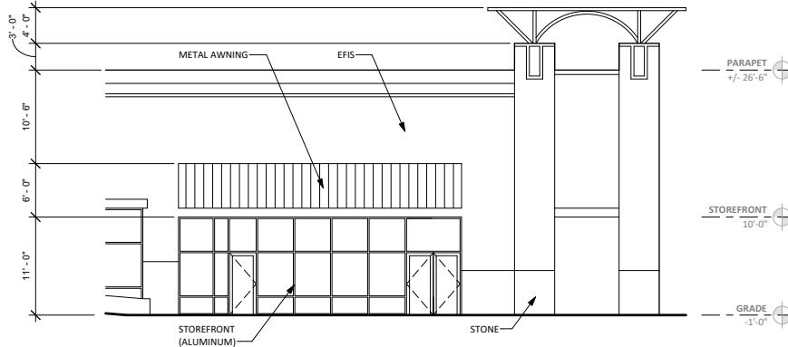
③ FRONT ELEVATION 1/8" = 1'-0"
