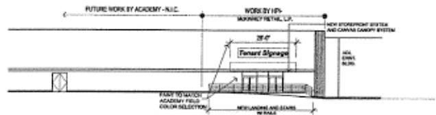
4 ELEVATIONS
